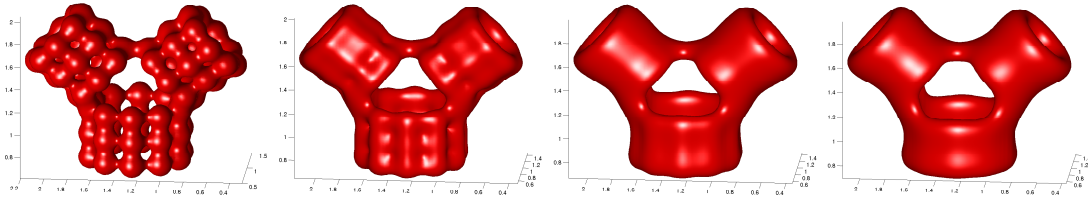
Figure 9: Perforated tube made via layer-by-layer deposition of cellular spheroids with a bad packing method. A defective branching vascular construct forms, in which holes are present in the branching point. Snapshots are taken at t = 0, 0.2, 0.4, 0.6 .
